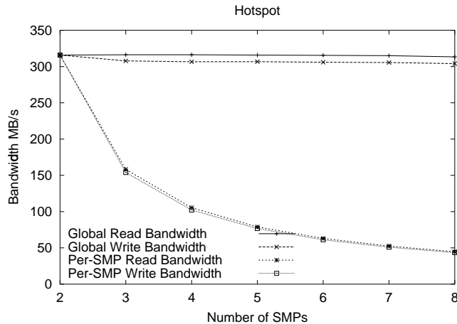
Figure 5. Read and Write Hotspot
