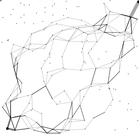
Fig. 4. Routing pattern of layer 10 built by the capillary routing algorithm on a network sample with 150 nodes
